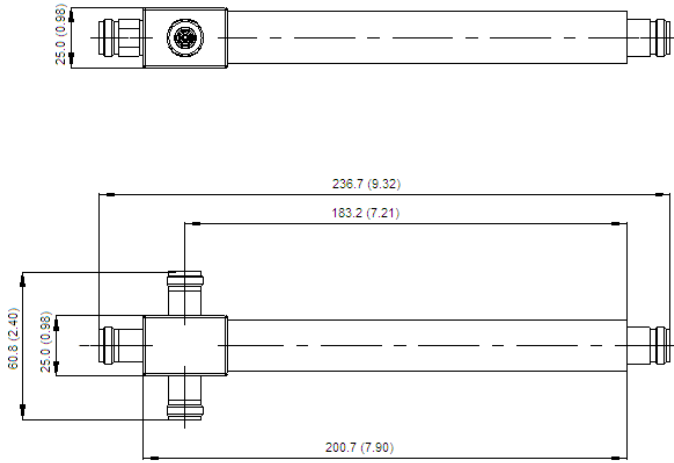
Dimensions mm(inch)
